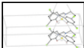
Fig. 2. Partial packing view showing the chain formed through C—H...O hydrogen bonds. H atoms not involved in hydrogen bondings have been omitted for clarity. H bonds are shown as dashed lines. [Symmetry code: (ii) -x + 1, y - 1, -z + 1/2 .]
